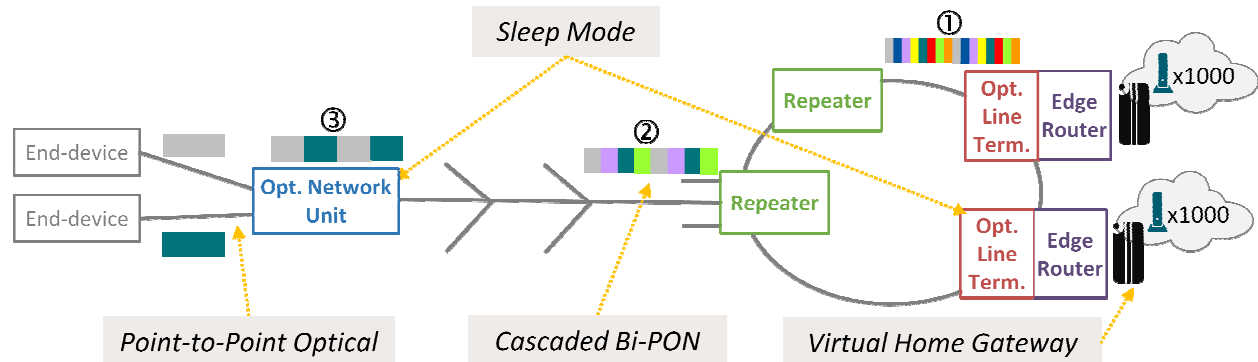
Figure 5: Network architecture of GreenTouch residential access network
