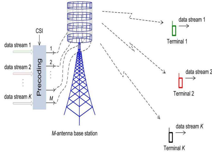
Figure 2: Large Scale Antenna System (LSAS) architecture
